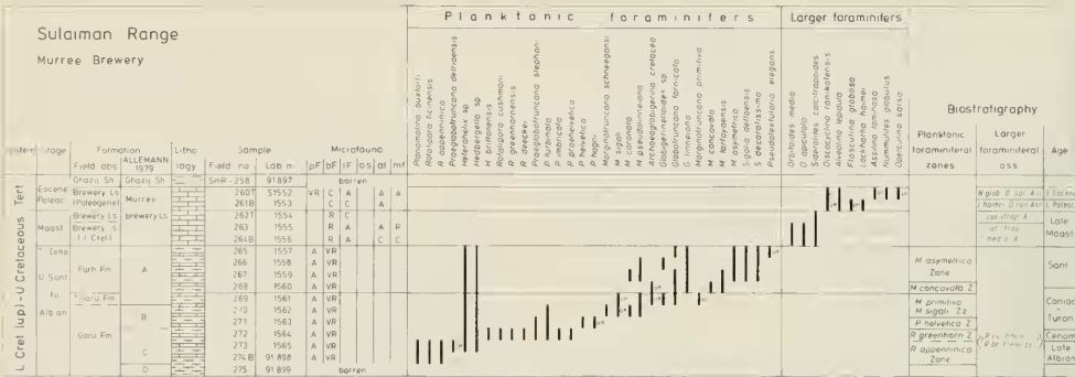
Fig. 11: Distribution of larger and planktonic foraminifers of the Murree Brewery Gorge section, Sulaiman Range. Abbreviations see Fig. 2.
